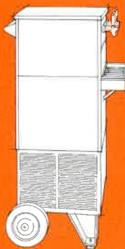
W-2 Two-Wheel Pushbar Kit. Two 8" rubber-tired wheels, plus two heavy-duty metal bracket legs; with attractive pushbar handle.
